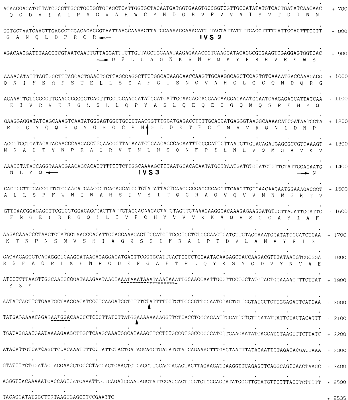
Fig.1. Nucleotide sequence (noncoding strand) and deduced amino acid sequence of a glutelin gene. Numbers are bp relative to the transcription start site. Consensus sequences (TATA box, enhancer core element and polyadenylation signals) are indicated by dashed lines. The legumin-box-like sequence is boxed. Direct repeat and CA-rich sequences are indicated by horizontal arrows and wavy lines. Arrowheads and vertical arrow indicate the poly(A) addition sites and the posttranslational processing site between the acidic and basic subunits.
